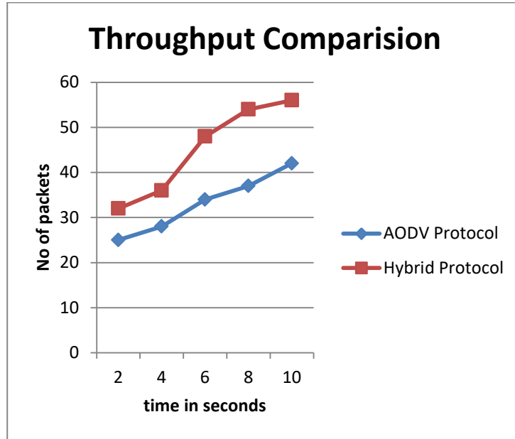
Fig 4: Throughput Comparison
